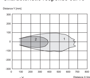
Kurve 1: flat surface 100 mm x 100 mm Kurve 2: round bar, \varnothing 25 mm
