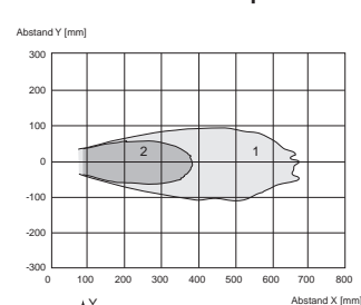
Kurve 1: ebene Platte 100 mm x 100 mm Kurve 2: Rundstab, \varnothing 25 mm
