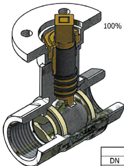
Regulation disc
